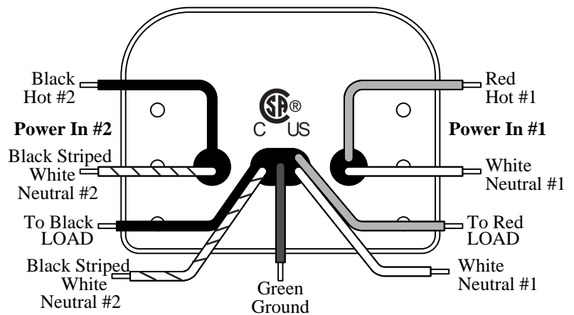
IPLC M210S Back Wiring Diagram (Backview)
